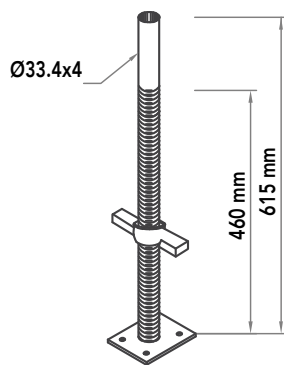
BASE JACK
