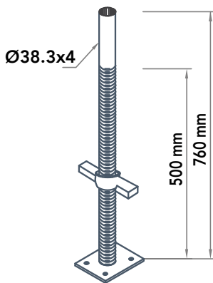
BASE JACK
