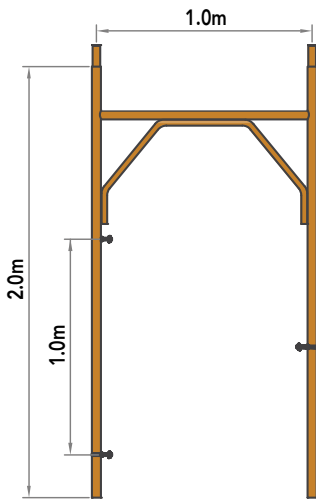
ITALIAN FRAME
