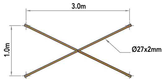
DIAGONAL BRACE
