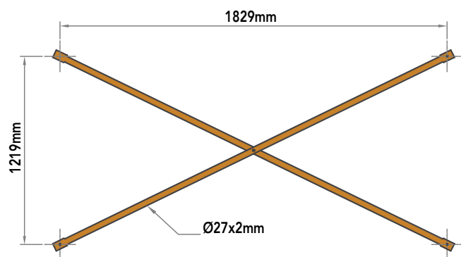
CROSS BRACE
