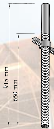
JACK
