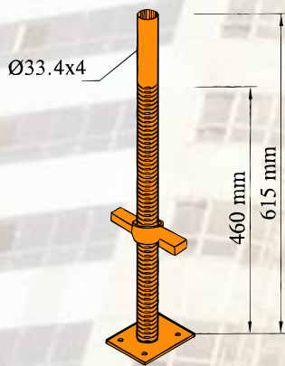
BASE JACK
